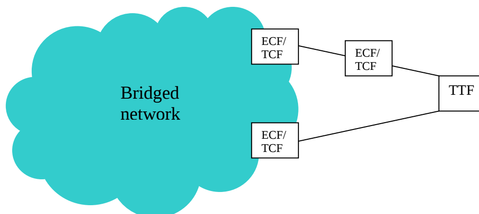
Figure 6: Link-redundancy
