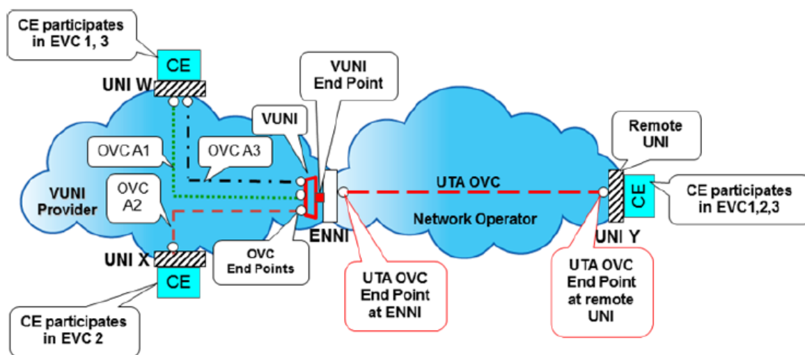
Figure 4 - Example of VUNIs (Figure 2 of MEF 28)
