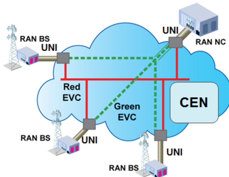
Figure 21: Ethernet Virtual Private Tree (EVP-Tree) Service
