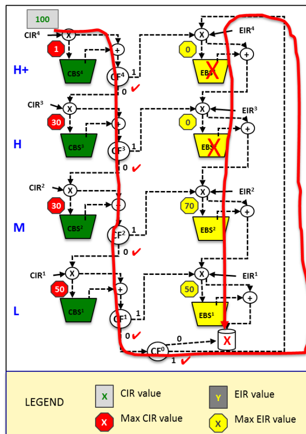
Figure 48: Example of token sharing for Mobile Backhaul
