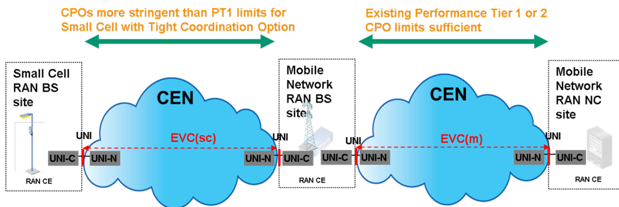
Figure 32: Two CPOs for Use Case 3
