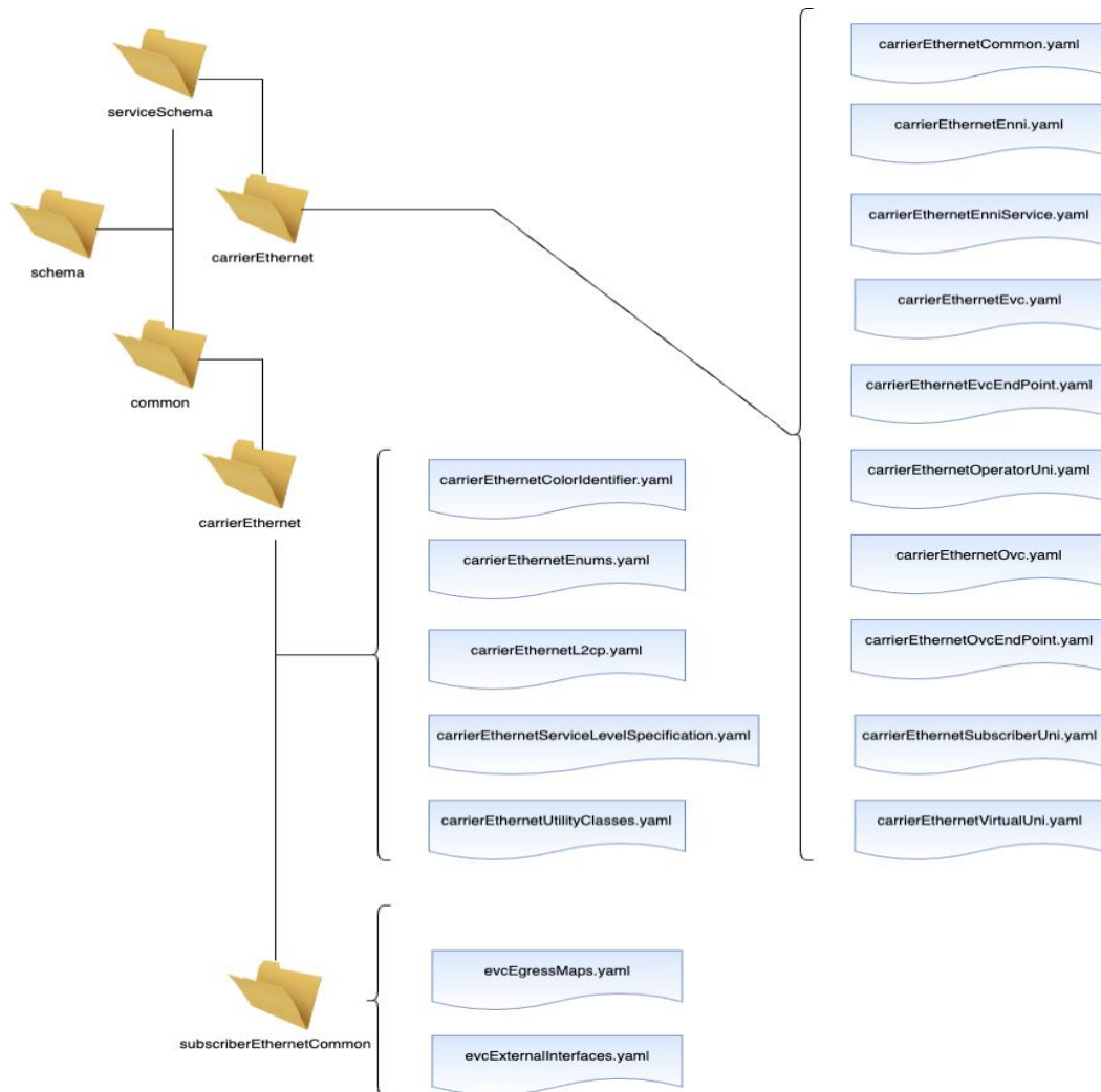
Figure 8-Schema Files Organization
