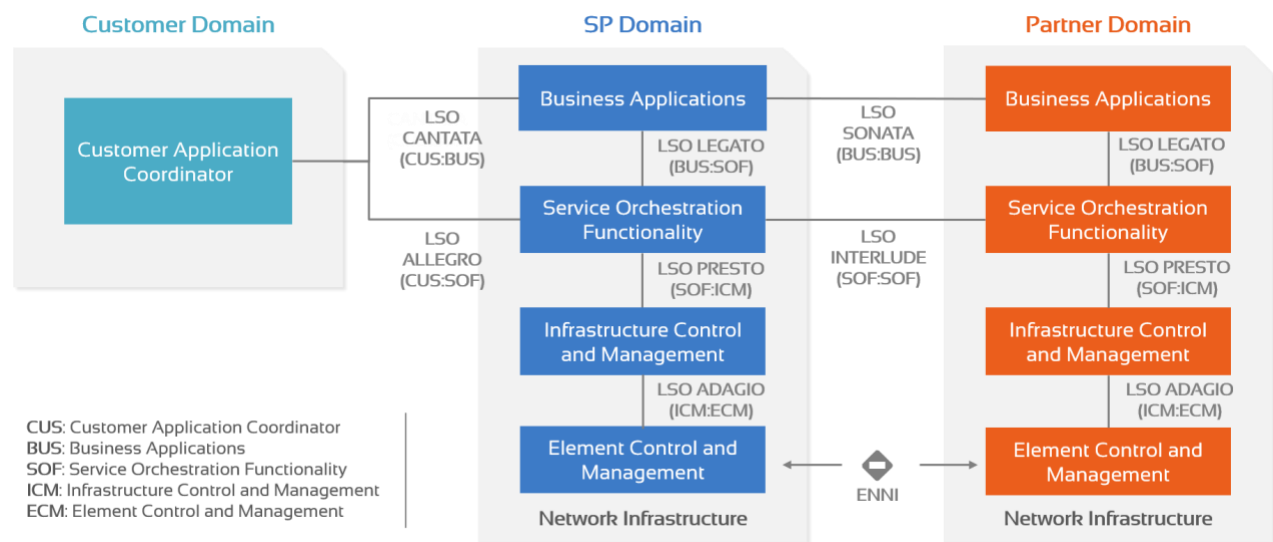
Figure 1-LSO Architecture Diagram
