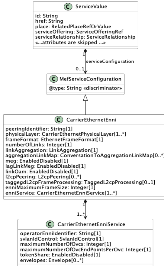
Figure 17-CarrierEthernetEnni Model
