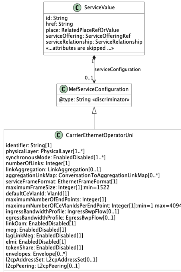
Figure 16-CarrierEthernetOperatorUni Model
