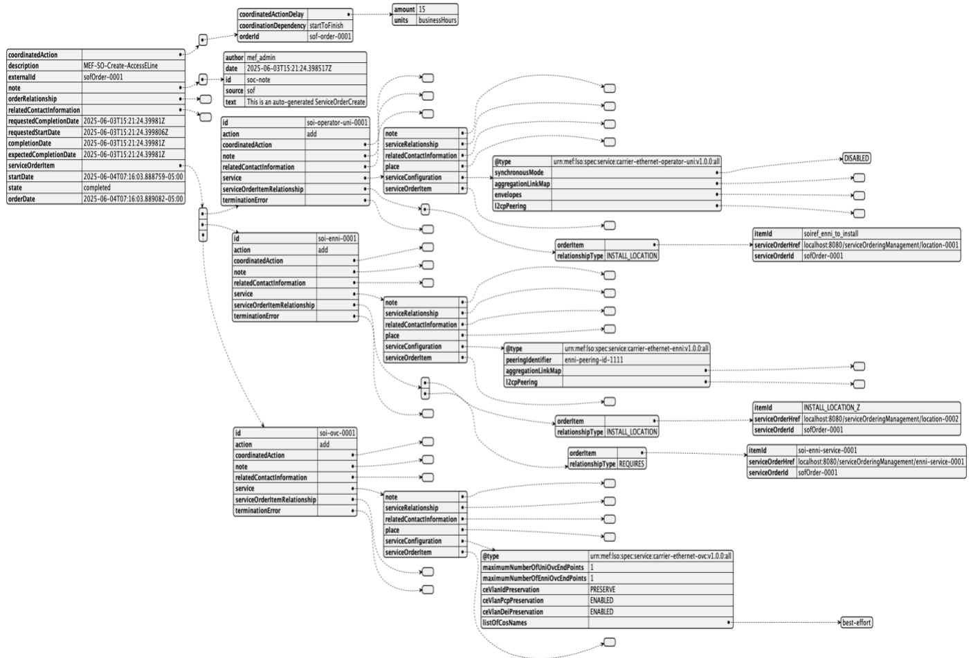
Figure 32-Service Order Response
