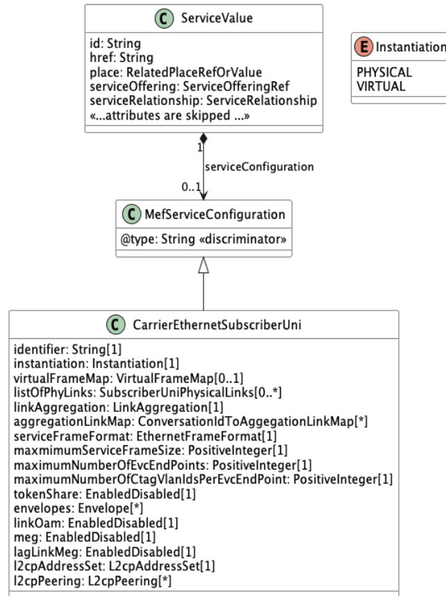
Figure 13-CarrierEthernetSubscriberUni Model
