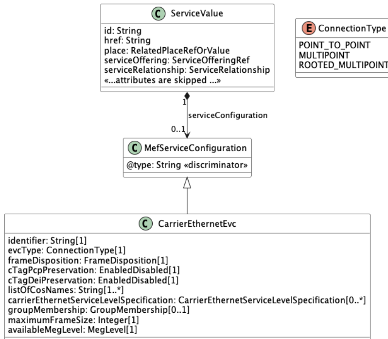
Figure 15-CarrierEthernetEvc Model
