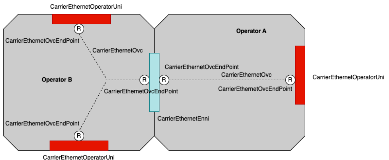
Figure 5-Operator Ethernet Service Topology
