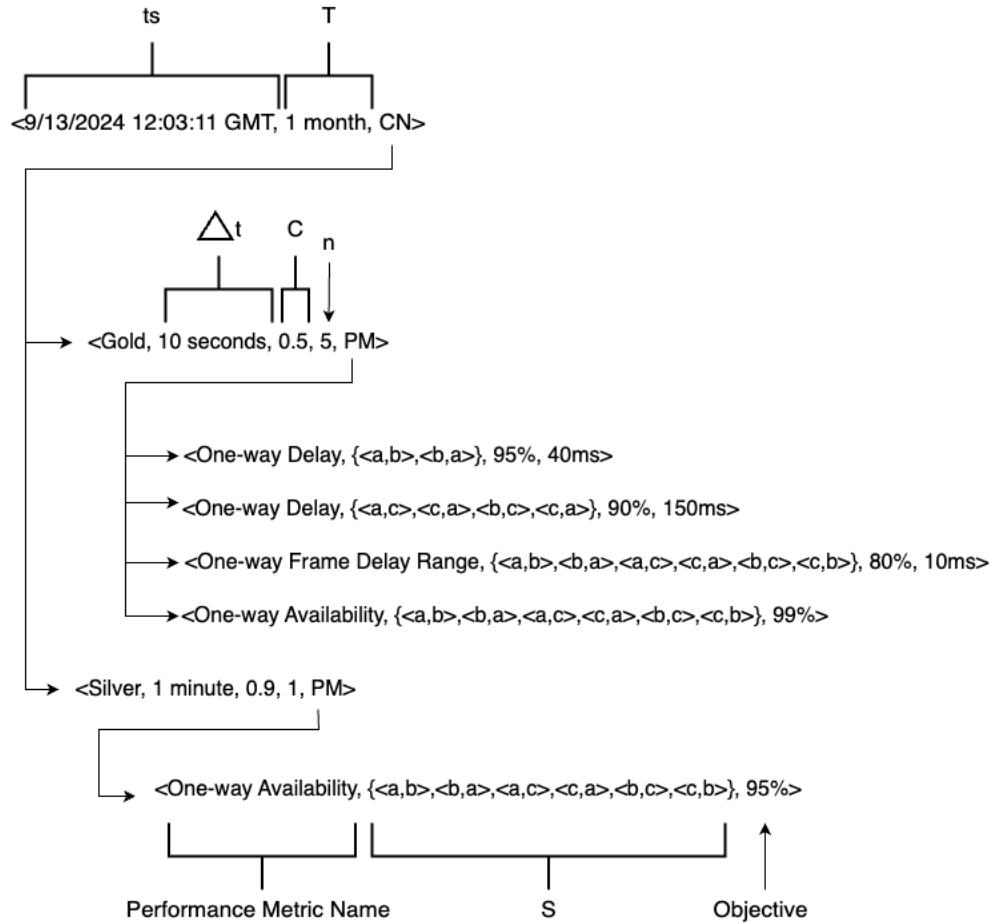
Figure 22-E/OVC Service Level Specification Service Attribute Value Example
