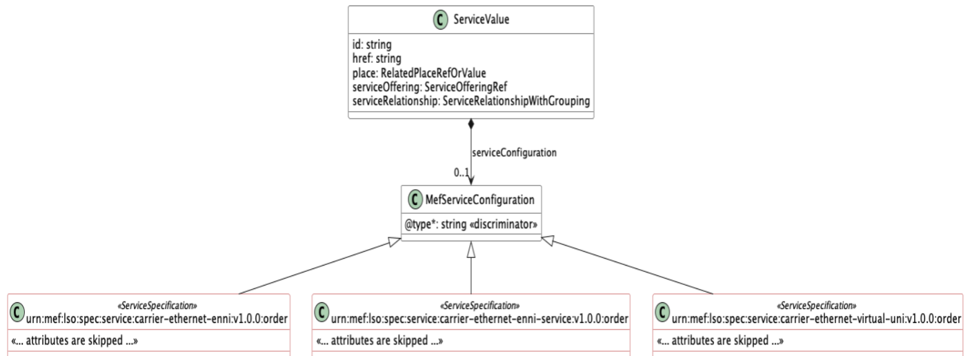
Figure 27-Extension Pattern: Operator Carrier Ethernet (2 of 2)
