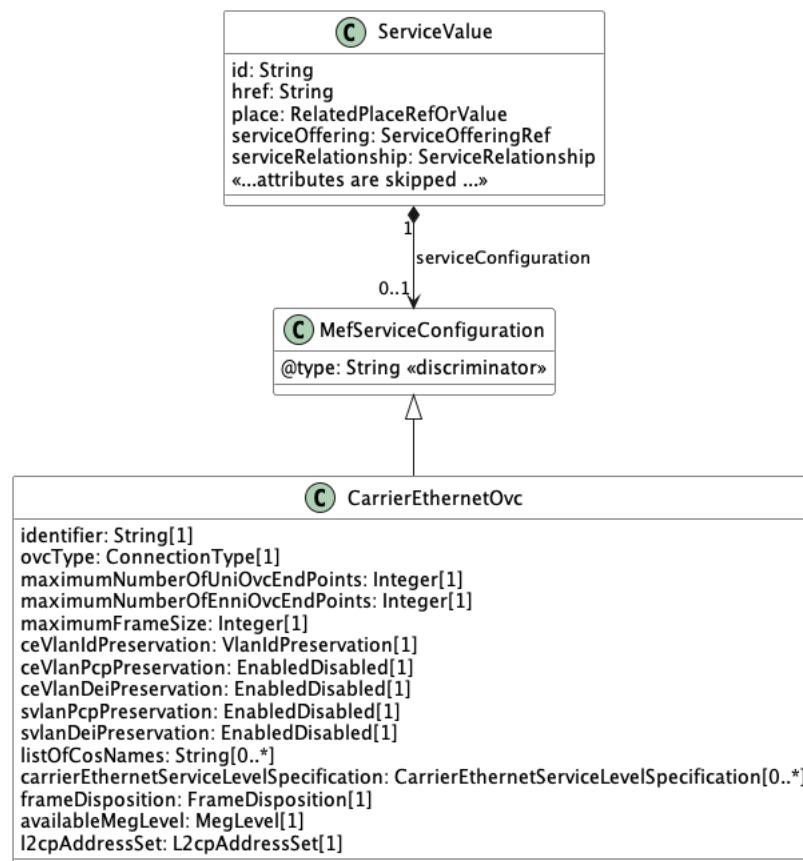
Figure 20-CarrierEthernetOvcModel
