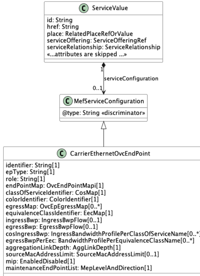
Figure 19-CarrierEthernetOvcEndPoint Model
